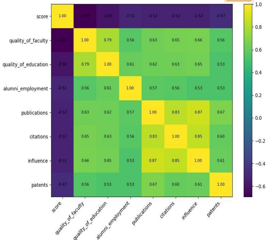
Figure 2: Correlation Heatmap of Key Variables
